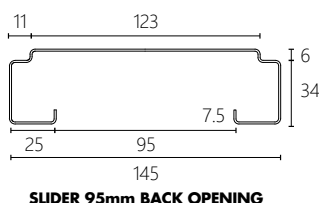
SLIDER 95mm BACK OPENING
