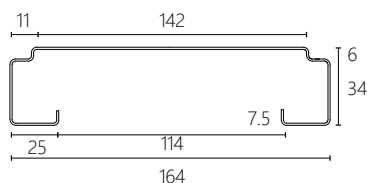
SLIDER 114mm BACK OPENING
