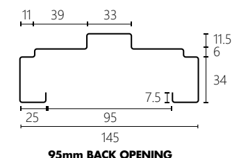
95mm BACK OPENING
