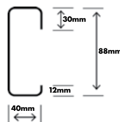
UNISPAN SECTION
