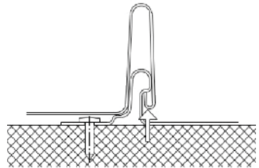
Concealed fix
