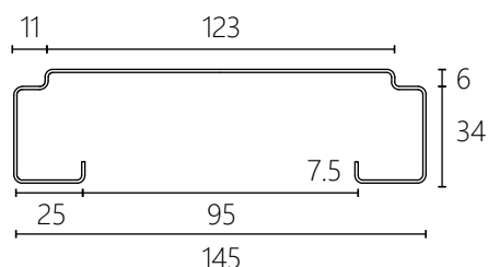
SLIDER 95mm BACK OPENING
