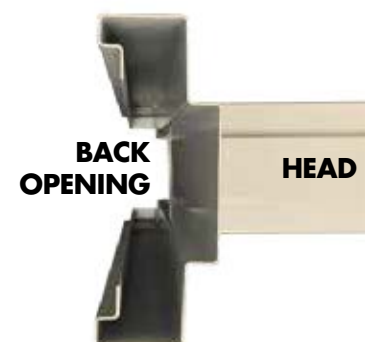
Sectional view from base up to head
