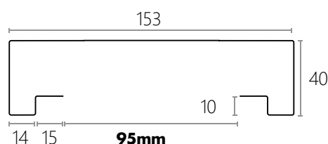
Sectional view from base up to head
