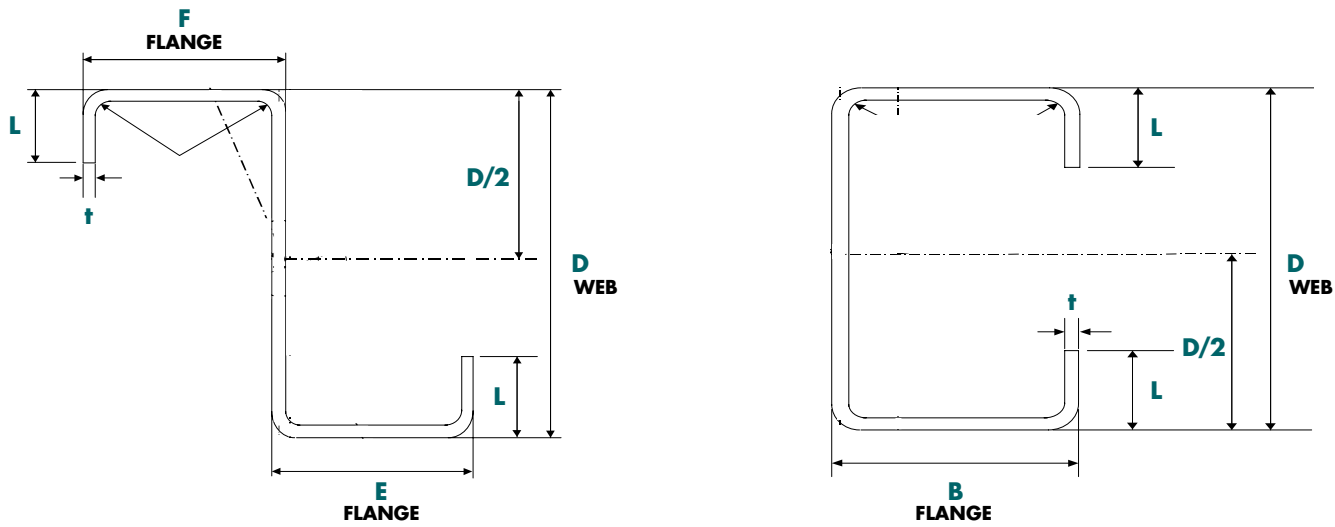
C & Z PURLIN SIZE & MASS TABLE
